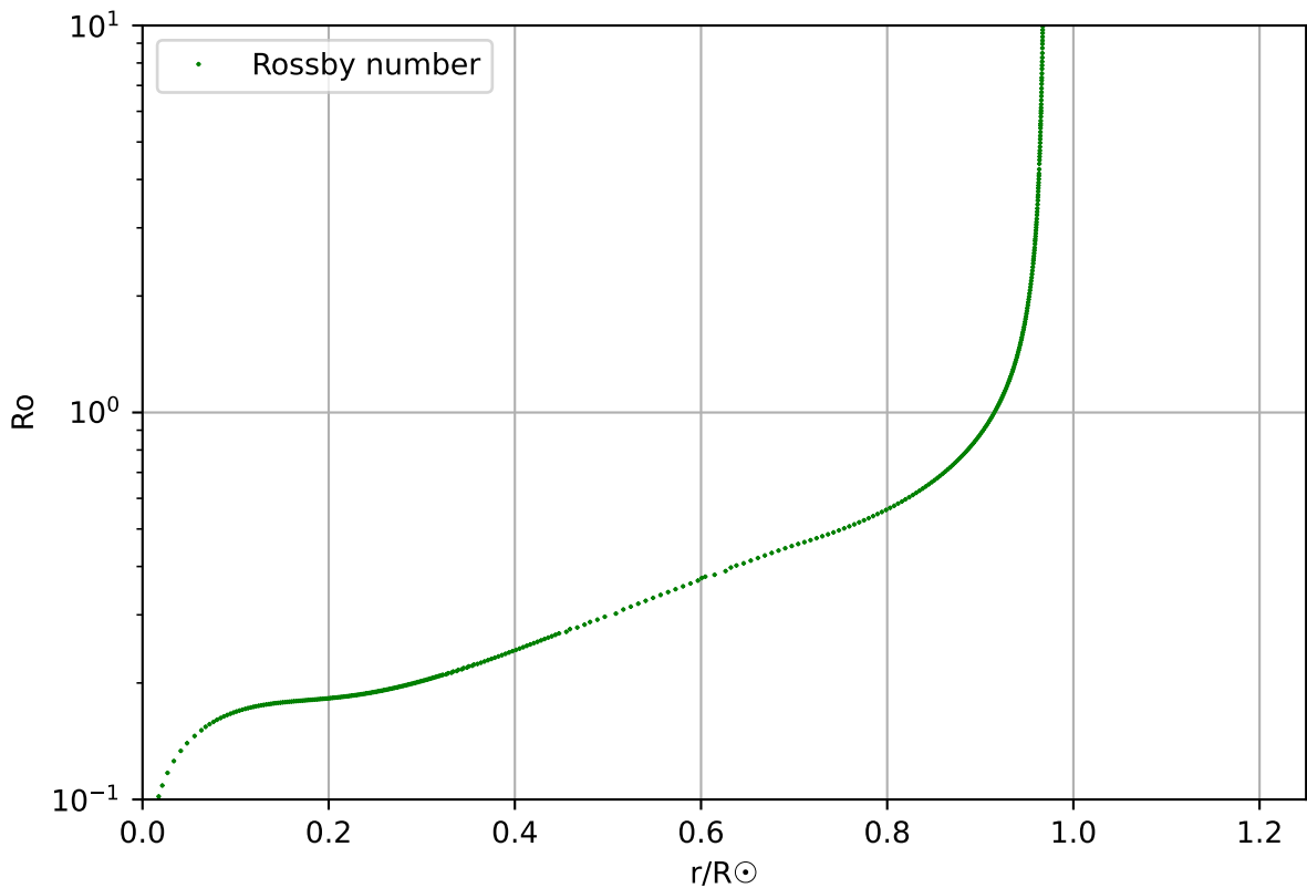
Rossby number, profile 143, age 3.71 \times 10^9
